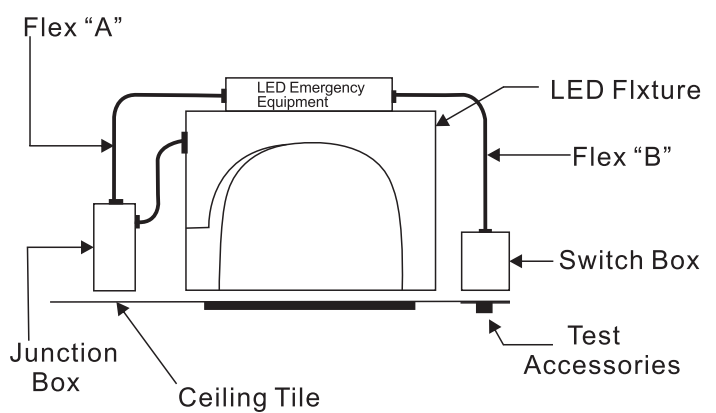
Illustration 1 Downlight Fixture
